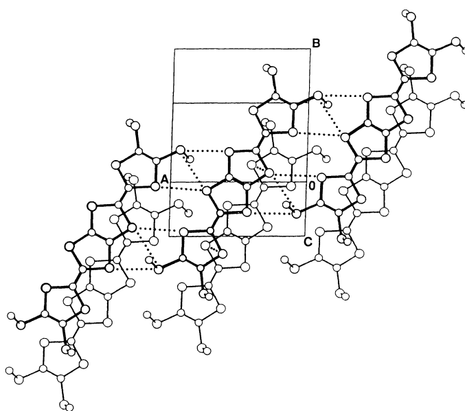
Fig. 2. Crystal structure of 1 showing close intermolecular contacts with dotted lines.
